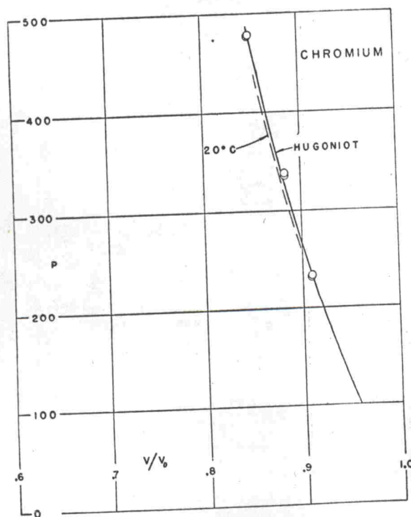
FIG. 6. Pressure-compression curves for chromium. See caption to Fig. 3.
